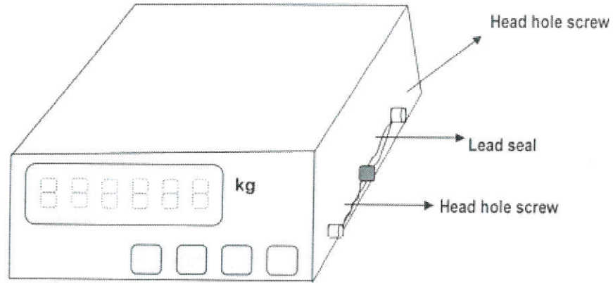
(Indicator of the Weighbridge — Front Side)
